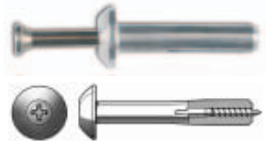
Zamac Hammer-Screw
