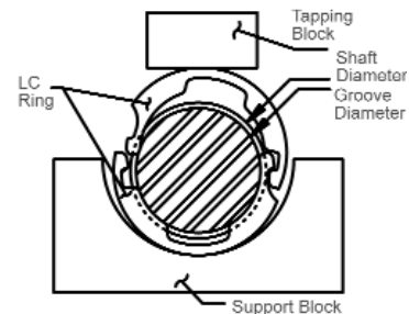
V-Block Assembly
