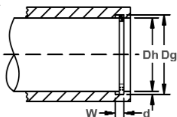
Housing Diameter & Groove Dimensions
